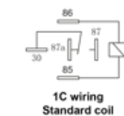
RE630C Miniature relay with insulating mounting bracket 24V, 20/10A, 1,6W 28 x 28 x 25,5 (+16) mm
